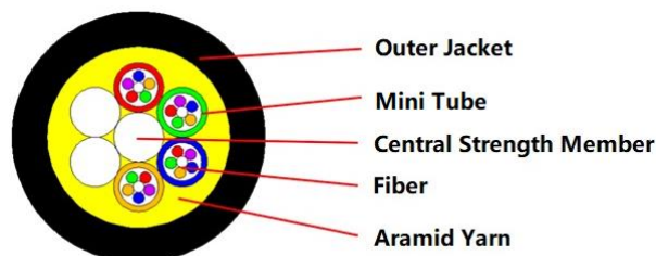
CABLE STRUCTURE AND PARAMETERS:
